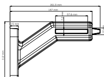
Part No. 900023/900025
