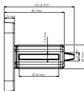
Part No. 900021-900022
