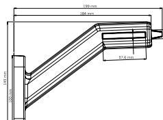
Part No. 900026-900027
