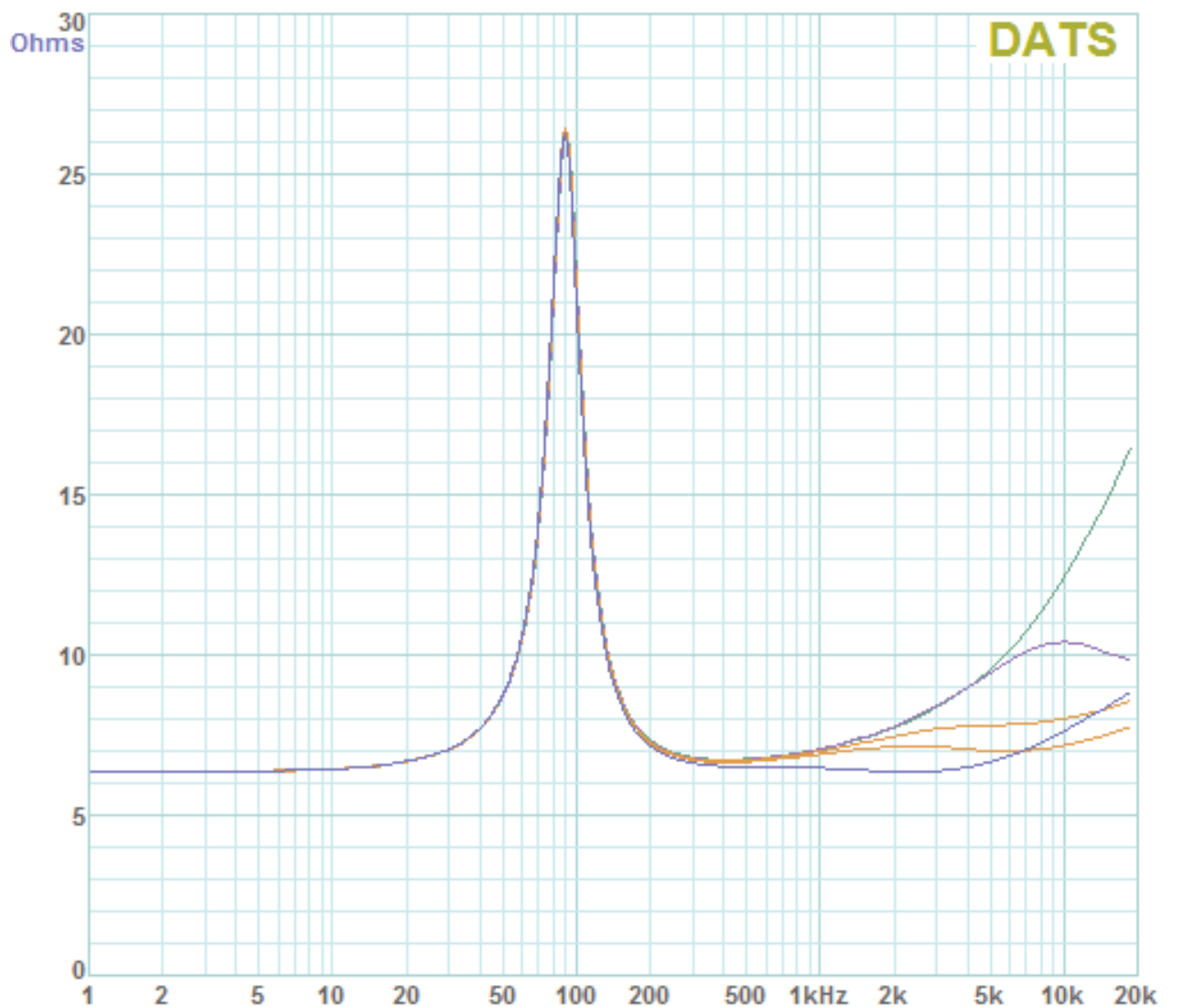
A 4" woofer in free air with Zobel network connected. R = 10 \text{ Ohms} C = 5 \text{ uF}
