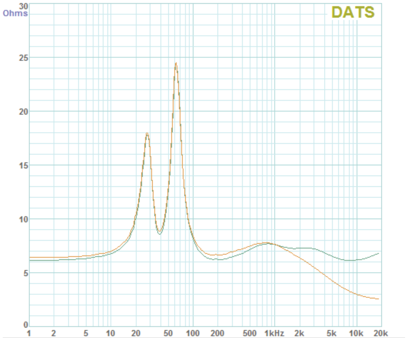
2-Way Vented Box Loudspeaker System The complete system: with tweeter "short circuited"
