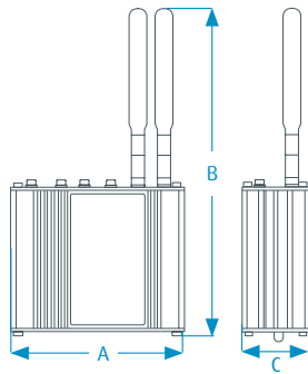
Roam Campervan X Router A: 115mm \varnothing B: 270mm C: 45mm Weight: 550g
