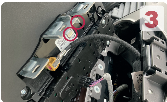
Slightly lift the unit and remove it from the dashboard. Remove the two connectors.
