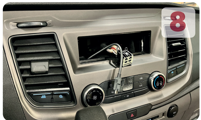
Remove the 1-Din radio or cover. Remove the frame from the dashboard.
