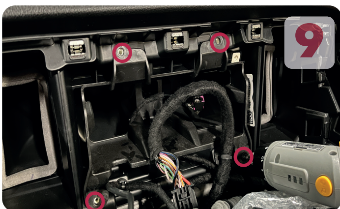
Remove four screws on the plastic support bracket.
