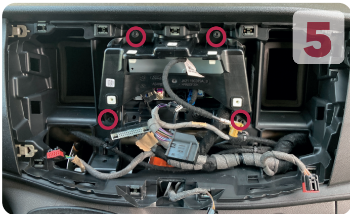
Remove four screws and take out the plastic support bracket.
